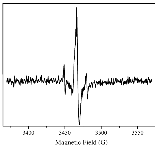
Fig. 4. Difference spectrum obtained by subtraction of Fig. 3a from d.
