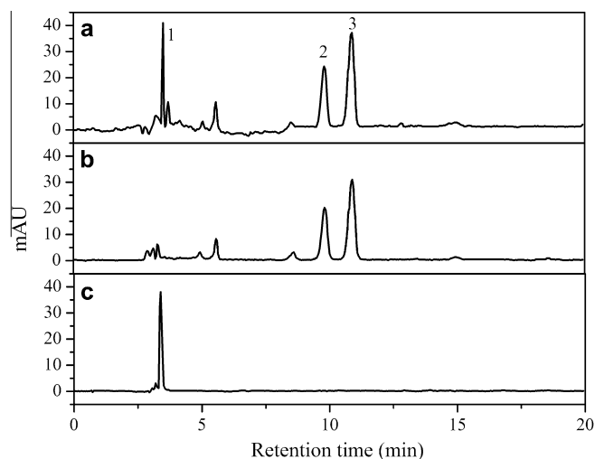
Fig. 1. HPLC chromatogram of pigments from macula. (a) Pigments extracted from macula by THF; (b) pigments extracted from macula by benzene; (c) standard retinal.
