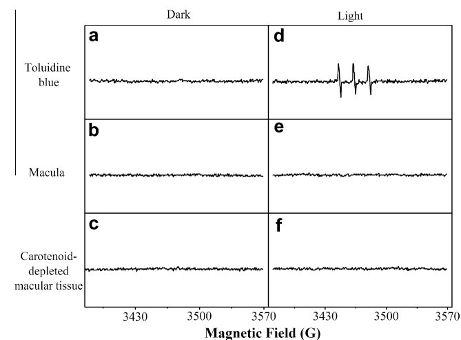
Fig. 2. EPR spectra of the singlet oxygen adduct TEMPO in macula. (a) Toluidine blue (1 mM), (b) macula, and (c) carotenoid-depleted macular tissue incubated with 80 mM TEMP under dark conditions; (d) toluidine blue (1 mM), (e) macula, and (f) carotenoid-depleted macular tissue incubated with 80 mM TEMP after 5 min of intense light treatment.
