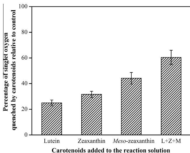
Fig. 5. Measurement of singlet oxygen quenching abilities of MP carotenoids by DMF assay. A 25 \mu l of each carotenoid (2 mM) stock solution was added to 1 ml of 0.2 mM DMF reaction solution in ethanol, and the absorption spectra at 215 nm were recorded on a spectrophotometer after the solution was illuminated for 5 min. The difference spectra between DMF and illuminated DMF solution were used as the control. The difference spectra between illuminated carotenoid solution and illuminated DMF solution were used to calculate the relative percentage of singlet oxygen quenched by each carotenoid.
