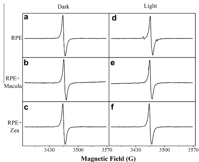
Fig. 3. EPR spectra of the singlet oxygen adduct TEMPO in foveal RPE. (a) Foveal RPE, (b) foveal RPE and macula, and (c) foveal RPE and 1 mM zeaxanthin incubated with 80 mM TEMP under dark conditions; (d) foveal RPE, (e) foveal RPE and macula, and (f) foveal RPE and 1 mM zeaxanthin incubated with 80 mM TEMP after 5-min light treatment.
